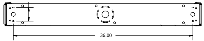
3' End Dimensions
