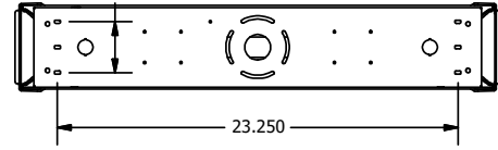
2' End Dimensions
