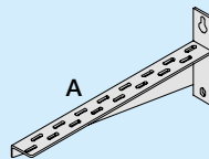
S280 Shelf Bracket A: 25.39" / 645 mm 316 St. Steel 570598 688280 4
